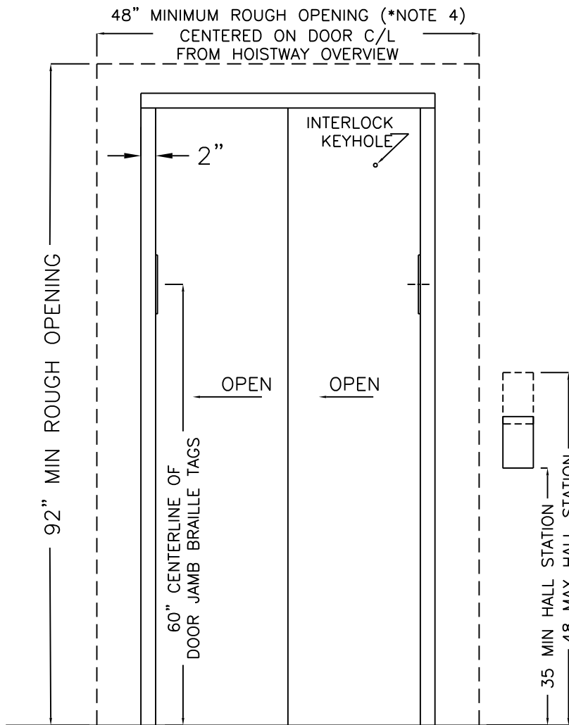
ENTRANCE ELEVATION TWO SPEED RIGHT HAND DOOR & ENTRANCE (FRONT)
